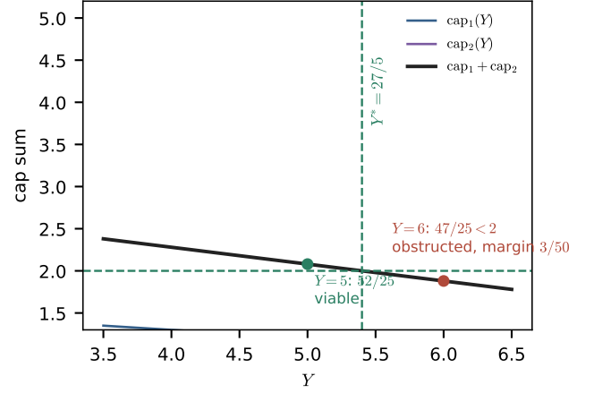
Figure 4: The benchmark. Both caps decrease linearly in the aggregate Y ; their sum crosses the demand level 2 exactly at Y^* = 27/5 . The Y = 5 fibre is viable (green), the Y = 6 fibre obstructed with margin 3/50 (red).
