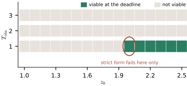
Figure 2: The timing grid. Cells viable at the deadline (green) satisfy T_{\text{obs}} \leq \tau^*(z_0) ; the identity is boundary-inclusive, and the strict form T_{\text{obs}} < \tau^*(z_0) fails at exactly one cell, (z_0, T_{\text{obs}}) = (2.0, 1) (circled); against the floored count \sigma^*(z_0) = \lfloor z_0 - 1 \rfloor the strict form fails on all six viable cells, which is why the inclusive predicate is the audited identity.
